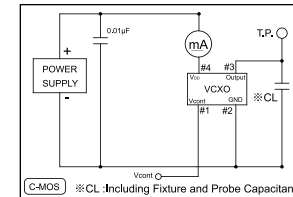
Measurement Circuit
