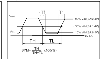
Output Waveform
