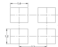
Recommended Land Pattern Tolerance: ±0.1
