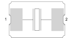
Internal Connection (Top View)
