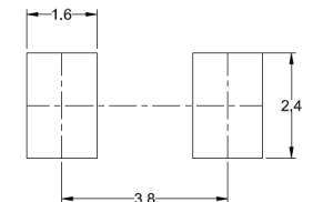
Recommended Land Pattern Tolerance: ±0.15
